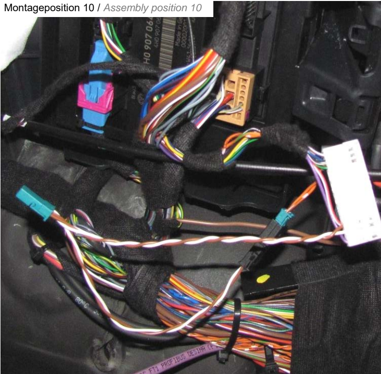
Montageposition 10 / Assembly position 10
