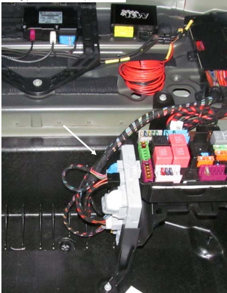
Montageposition 11 / Assembly position 11
