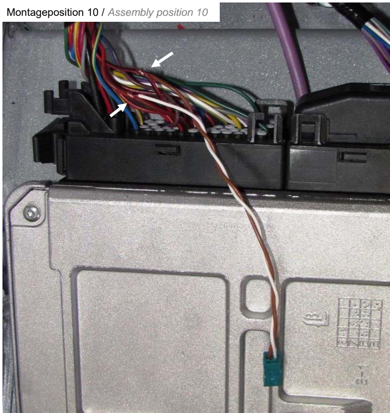
Montageposition 10 / Assembly position 10
