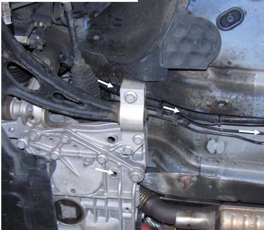
Montageposition 2 / Assembly position 2
