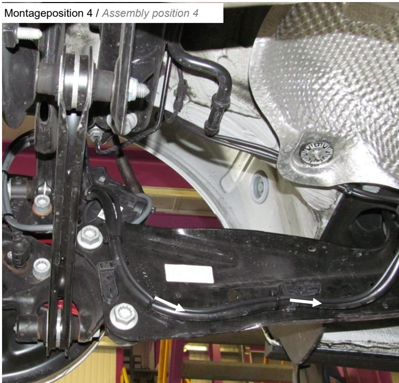
Montageposition 4 / Assembly position 4
