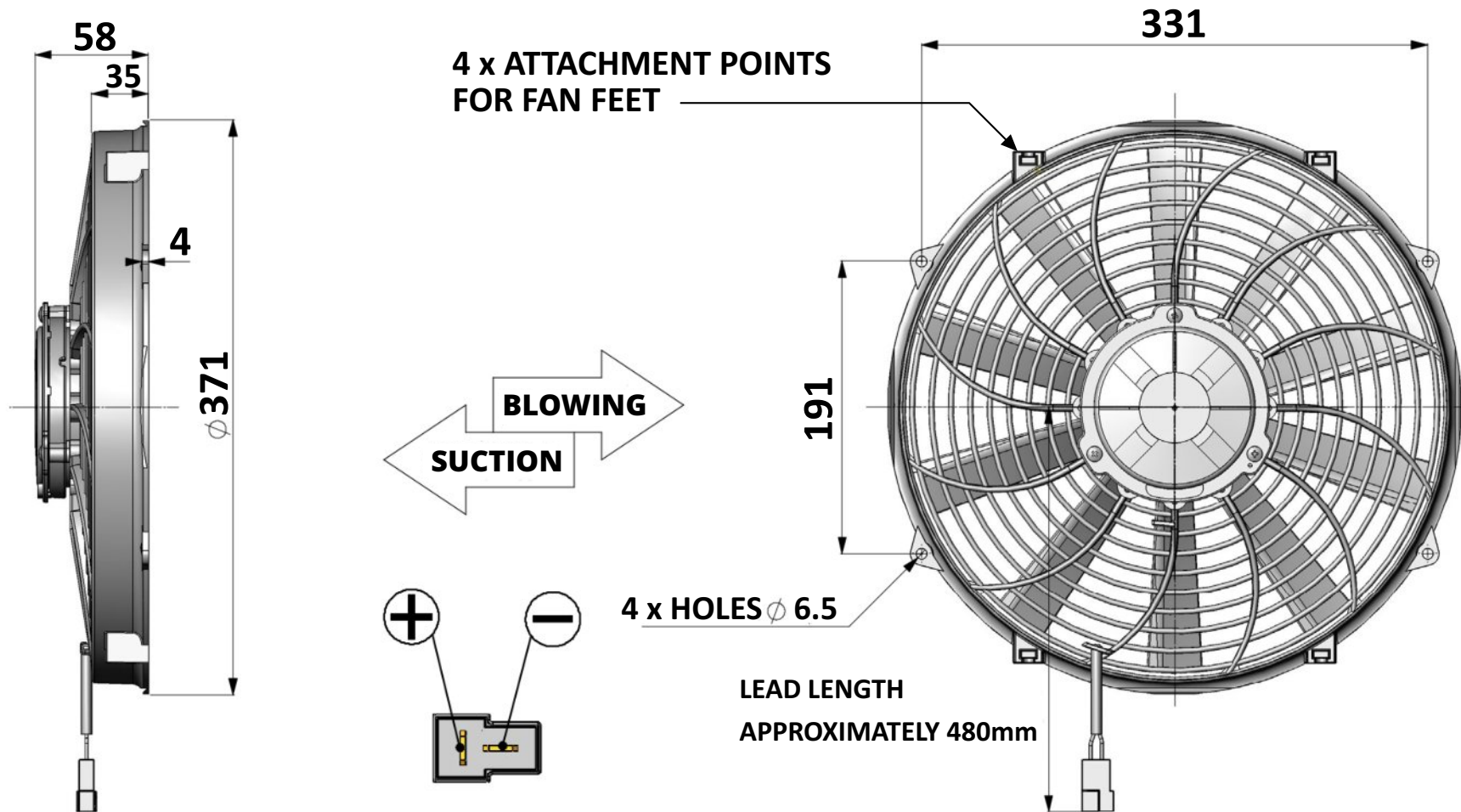
FAN FITTED WITH FEMALE CONNECTOR: TYPE TYCO CODE 180908-0 (MALE CONNECTOR: REVOTEC RTB-2)
